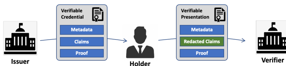
Figure 7 - Verifiable Credentials
