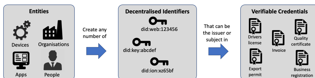
Figure 8 - Decentralised Identifiers
